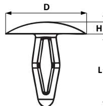
1-1690BLK Canoe clip • Black finish 7.4mm D x 2.5mm H x 5.5mm L. Use 5/32" drill bit.
