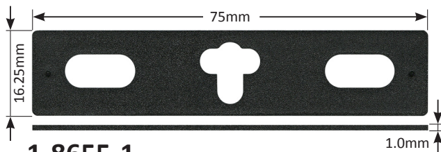
1-8655-1 Spacer • Suit striker plate or hinge 1mm thick. Black plastic. Includes stacking pips.
